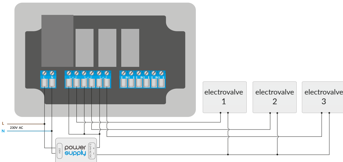
Diagram of low voltage connection (e.g. control of 5V-24V AC / DC solenoid valves):
